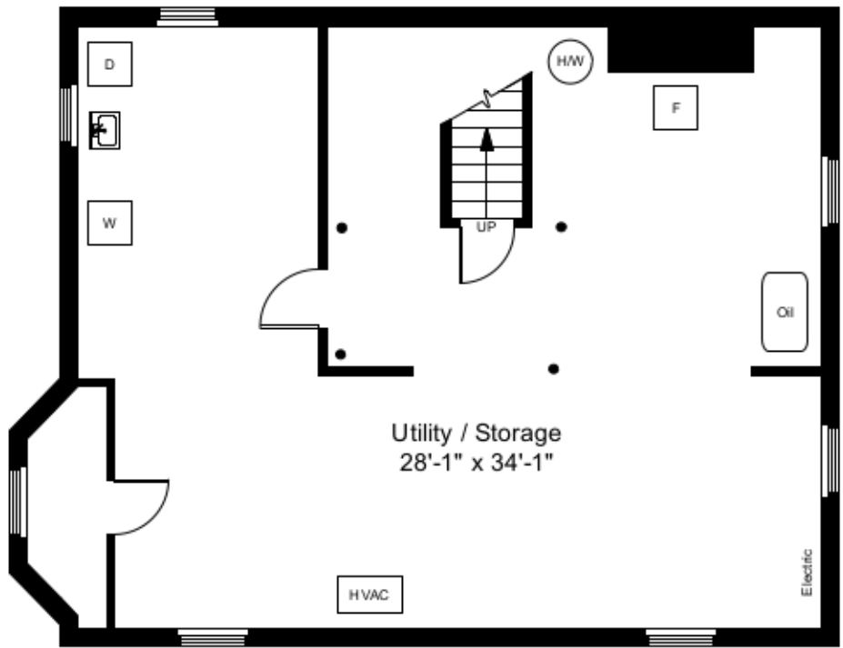
Basement Plan Ceiling Height = 7'-5"
