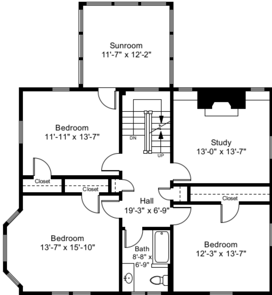
Second Floor Plan Ceiling Height = 7'-11"
